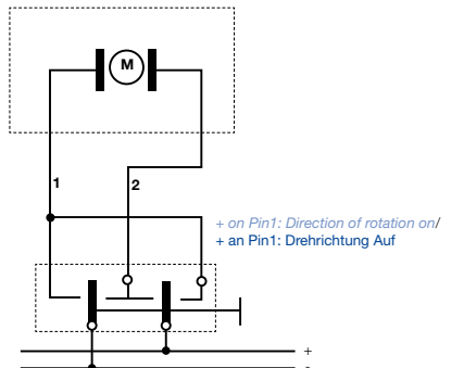
Drives/ Antriebe: DCD22 | DCD55
